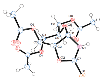
Figure 1. ORTEP (ellipsoids at 50% probability) view of the X-ray structure of 7 .
